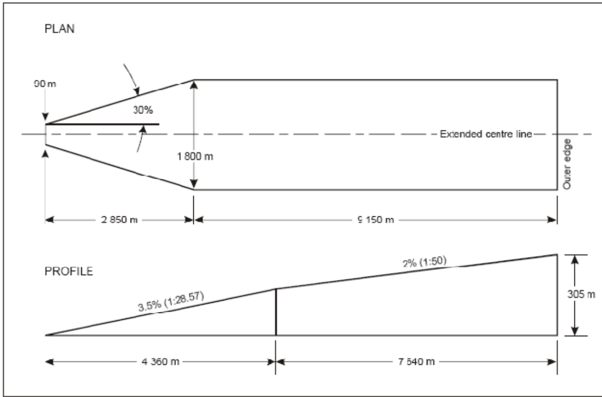
Figure 4-5. Take-off climb surface for instrument FATO
