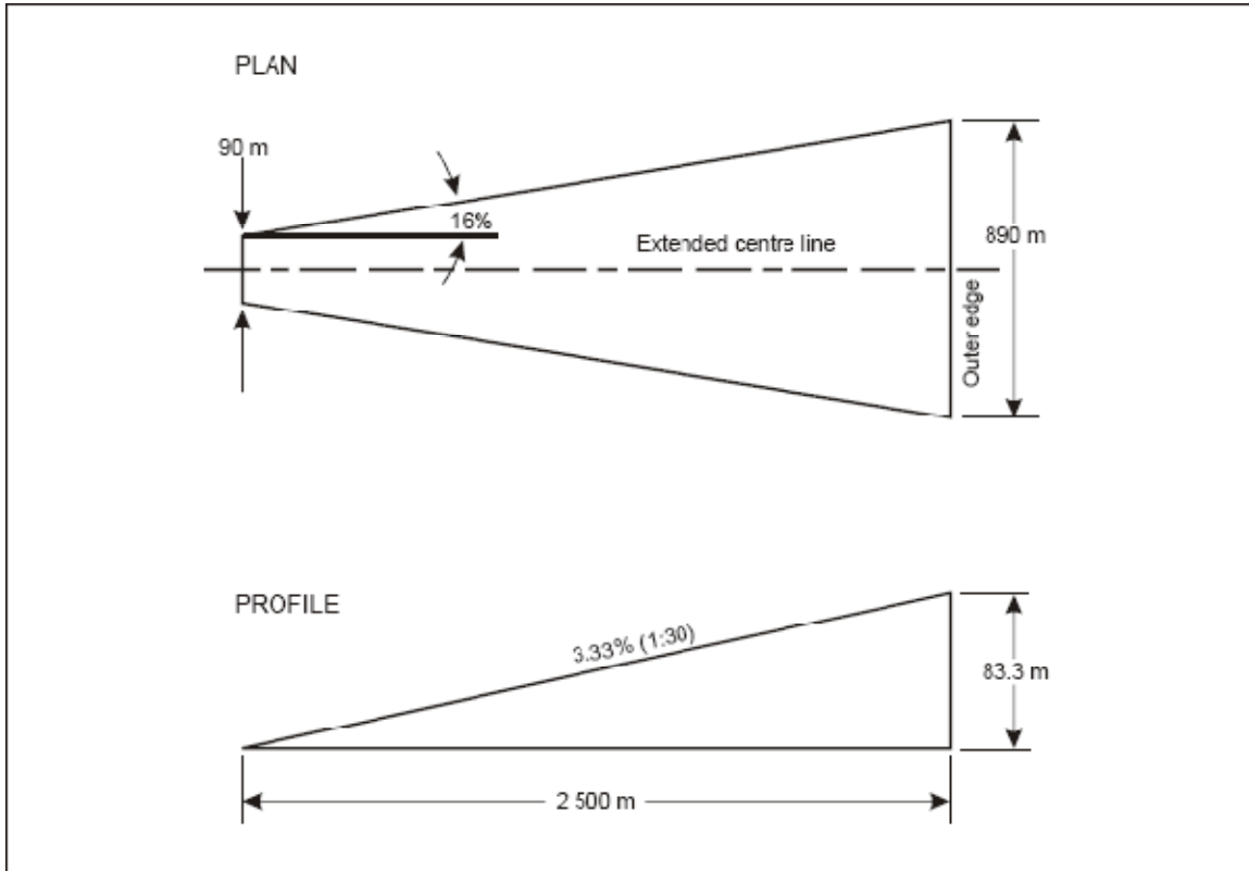
Figure 4-7. Approach surface for non-precision approach FATO
