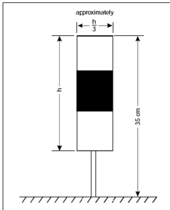
Figure 5-6. Air taxiway marker
