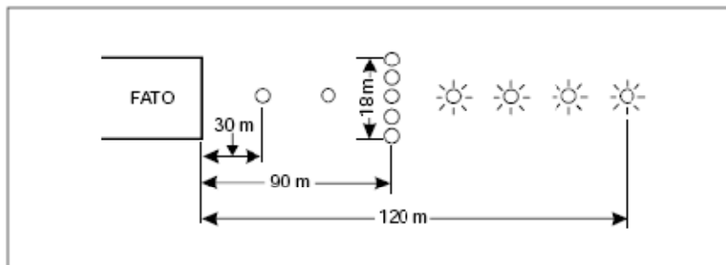
Figure 5-10. Approach lighting system
