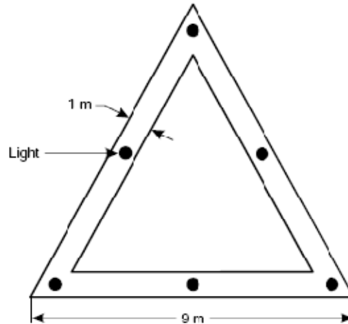
Figure 5-4. Aiming point marking
