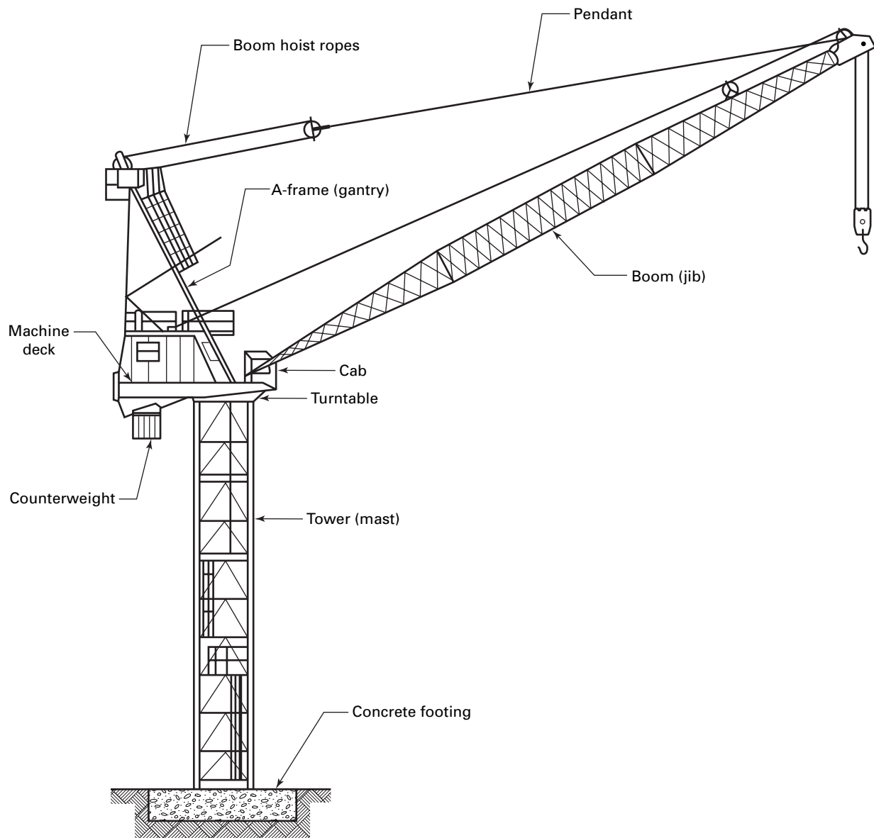
Fig. 3-0.2.1.2-3 Luffing Tower Crane — Fixed-Base, Free-Standing Crane
