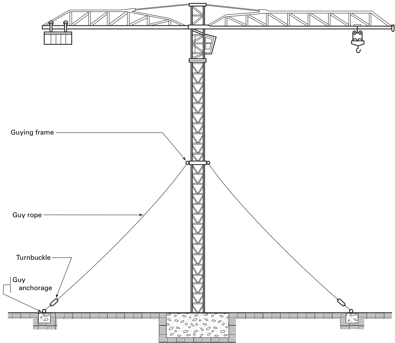
Fig. 3-0.2.1.2-2 Guyed Tower Crane
