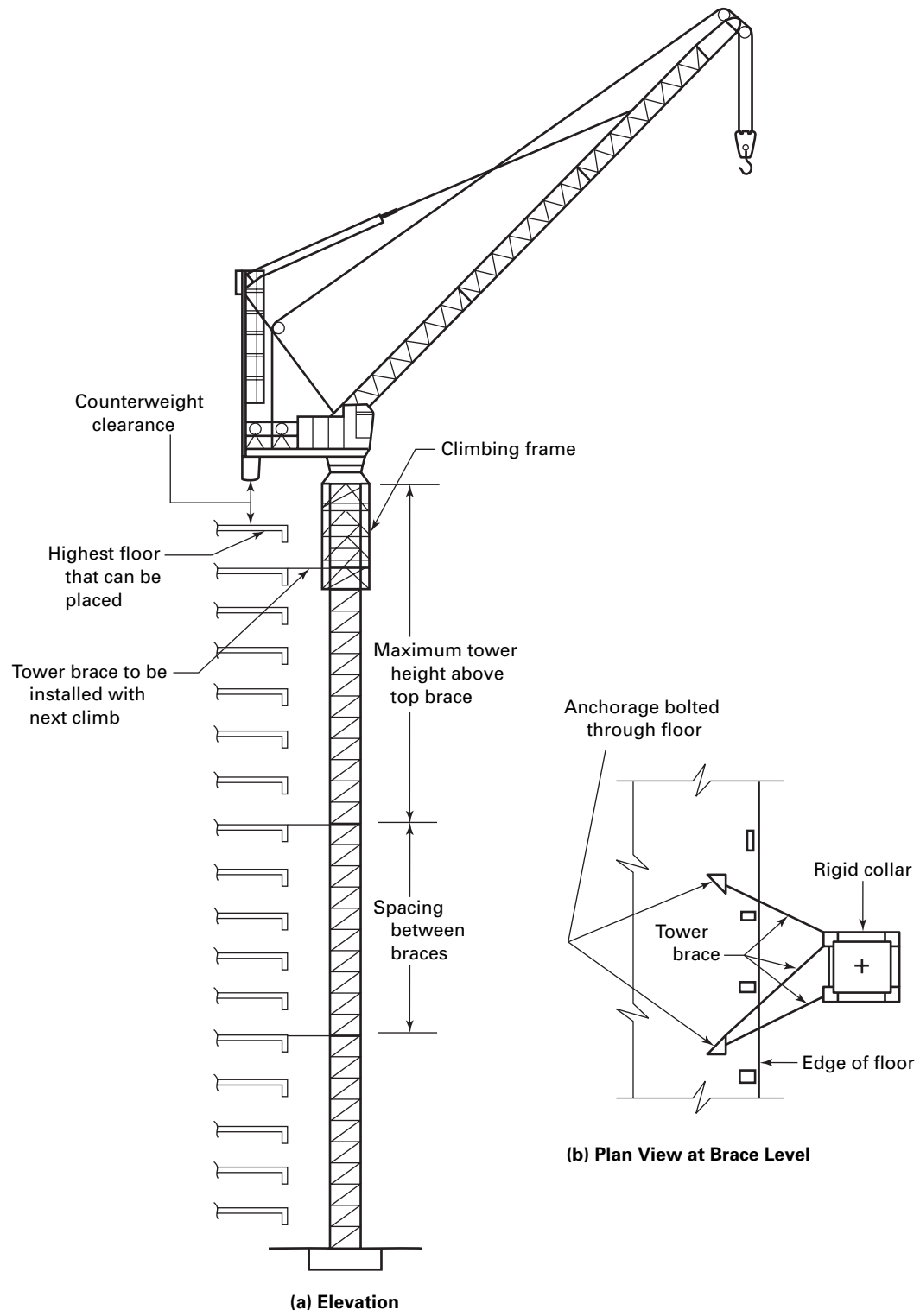
Fig. 3-0.2.1.2-4 Braced Crane
